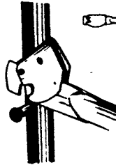
SNAP-ON GUARD RAILS 3' 5' 7' 10' Can be manufactured to any size
